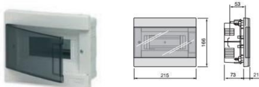
V52408 8 modules, delivered with DIN rail (60715 TH35), RAL 9003 white, with transparent door, fumé. Dissipated power: 19 W
