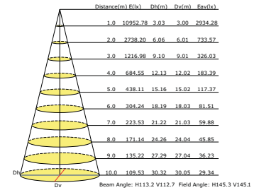
Illuminance at a Distance
