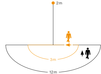
IS 2180-2 detection zone (12 m lens) Possible mounting height: 1.8-4 m Orange: radial Black: tangential
