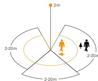
Detection zone for sensIQ Possible mounting height: 2-5 m Orange: radial Black: tangential 3 scalable zones
