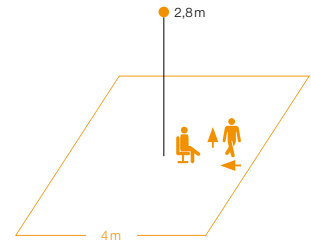
IR Quattro SLIM detection zone Possible mounting height: 2.5 - 4 m Orange: presence, tangential and radial
