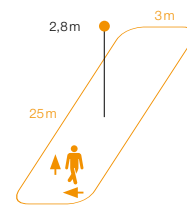
Hallway detection zone Possible mounting height: 2-4 m Orange: radial and tangential
