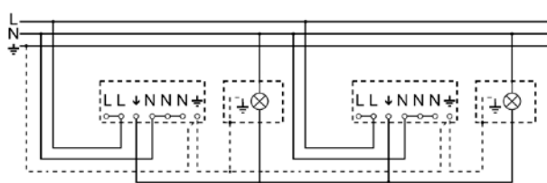
Master/slave
