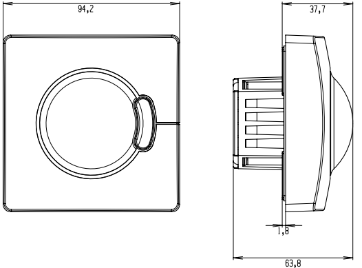
Concealed installation, square
