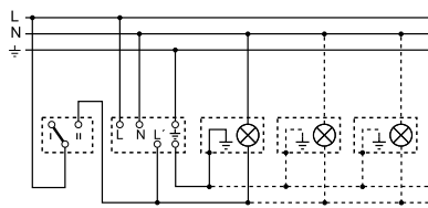
Connection via a two-way switch
