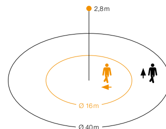
IS 3360 detection zone Possible mounting height: 2.5 - 4 m Orange: radial Black: tangential
