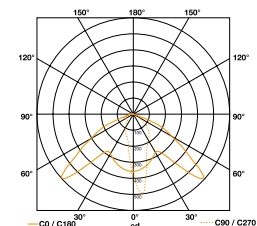
Light distribution curve for XLED PRO Wide
