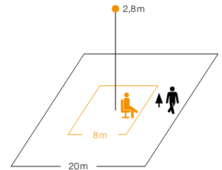
IR Quattro HD detection zone Possible mounting height: 2.5 - 10 m Orange: presence and radial Black: tangential
