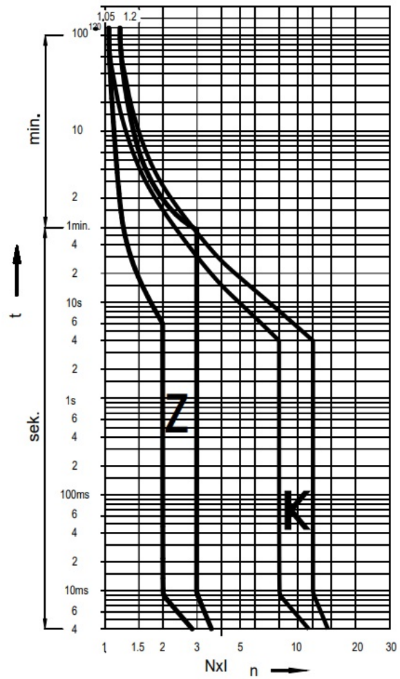
I/t characteristic at 50 and 60Hz
