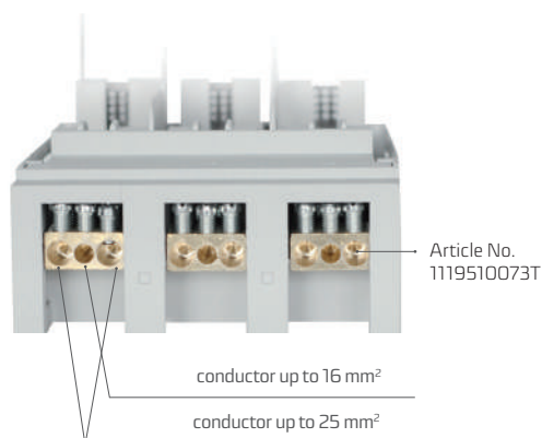
RBK 00-W with terminal clamp 1x16 mm 2 , 2x25 mm 2 (view of fuse switch disconnecter without fuse-link cover)
