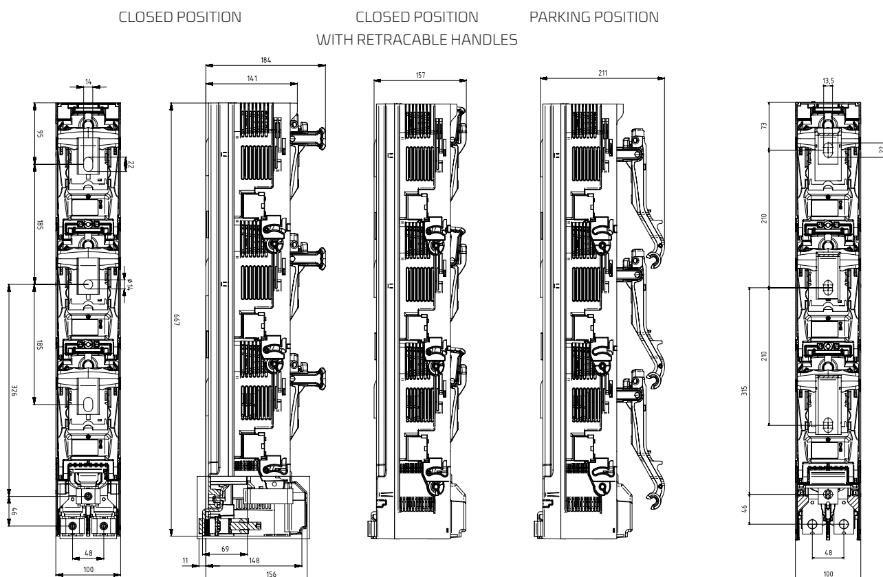
smartARS 2 P pro, smartARS 3 P pro 1-phase
