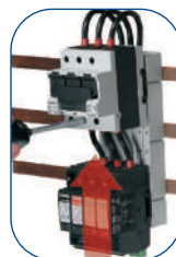
Side element, width 9 mm allows to expand adapter base by 9 mm
