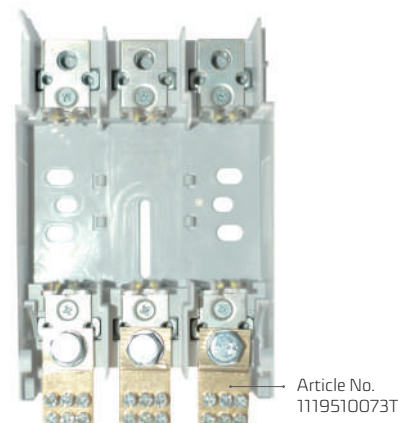
RBK 00-W with terminal clamp 1x16 mm 2 , 2x25 mm 2 (view of fuse switch disconnecter without fuse-link cover and terminal shrouds)
