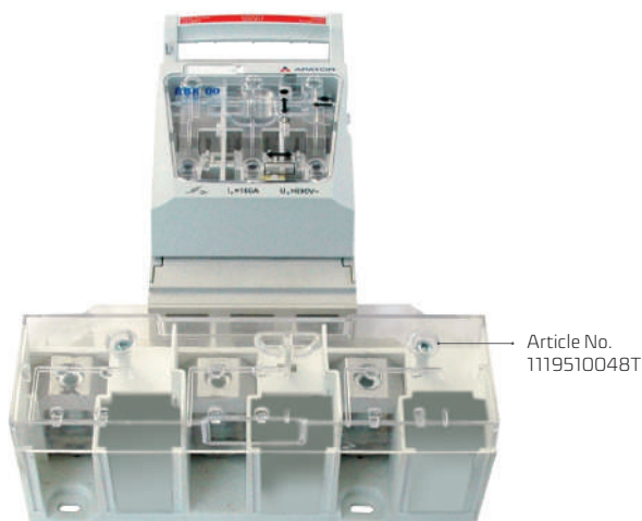
RBK 00-W with terminal adapter for connection of sector-shaped conductors with cross-section up to 240 mm 2
