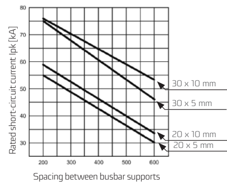
Short-circuit resistance diagram according to DIN EN 60439 60 mm busbar system Rated operating voltage: 690 V, Rated frequency: 50 Hz
