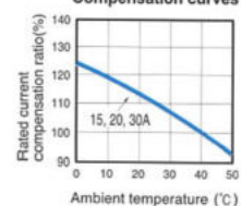
Compensation curves
