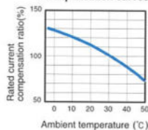
Compensation curves
