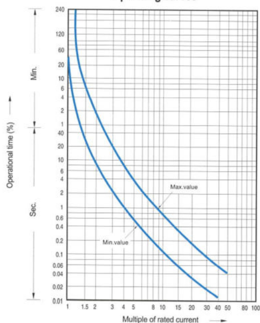
Operating curves
