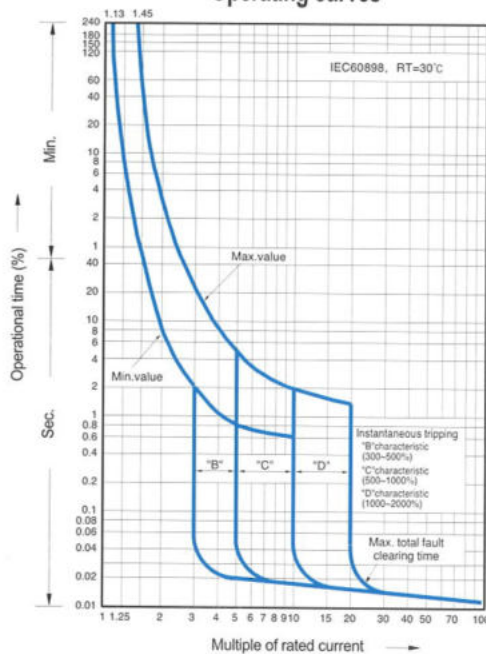
Operating curves
