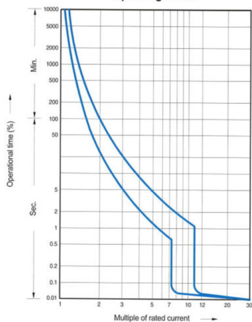
Operating curves
