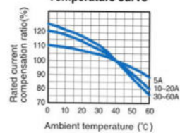
Temperature curve
