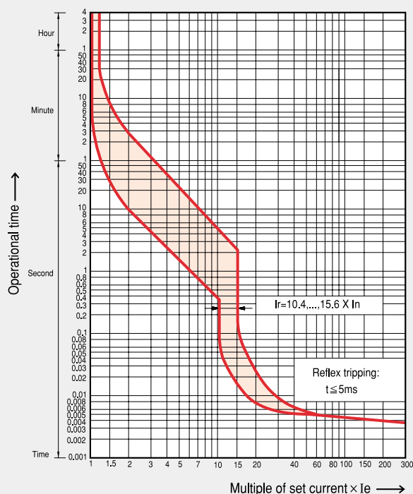
MMS-32AF Tripping Curve
